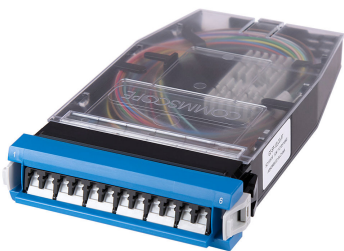
G2 Splice Cassette, 12LC/UPC with internal shutters, OS2, with 250um pigtails
